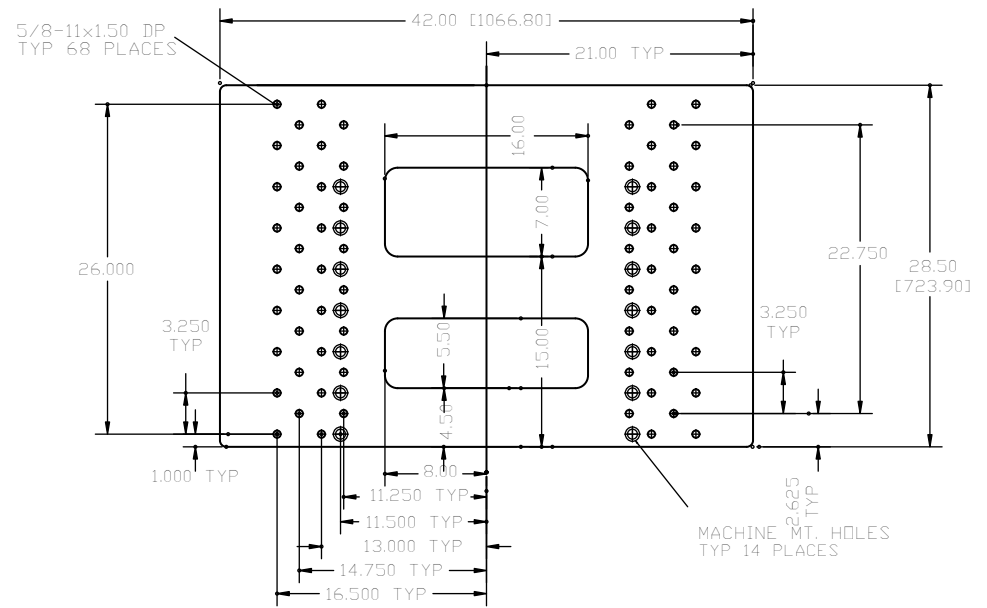
PLATEN, 2.00" MOVABLE
