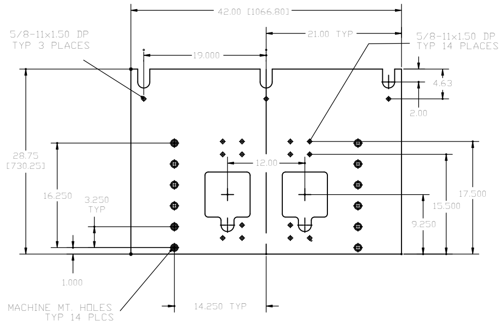
PLATEN, 2.00" REAR
