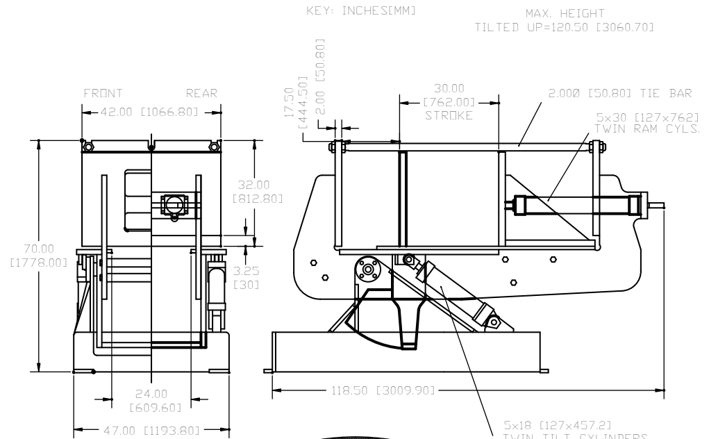
PLATEN, 2.00" MOVABLE
