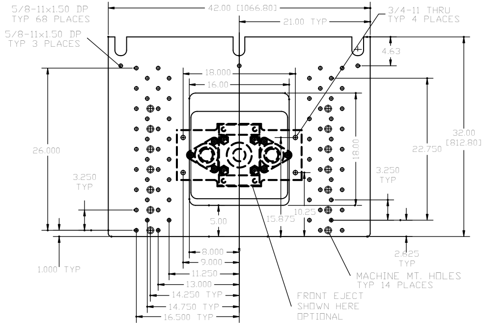
PLATEN, 2.00" FRONT
