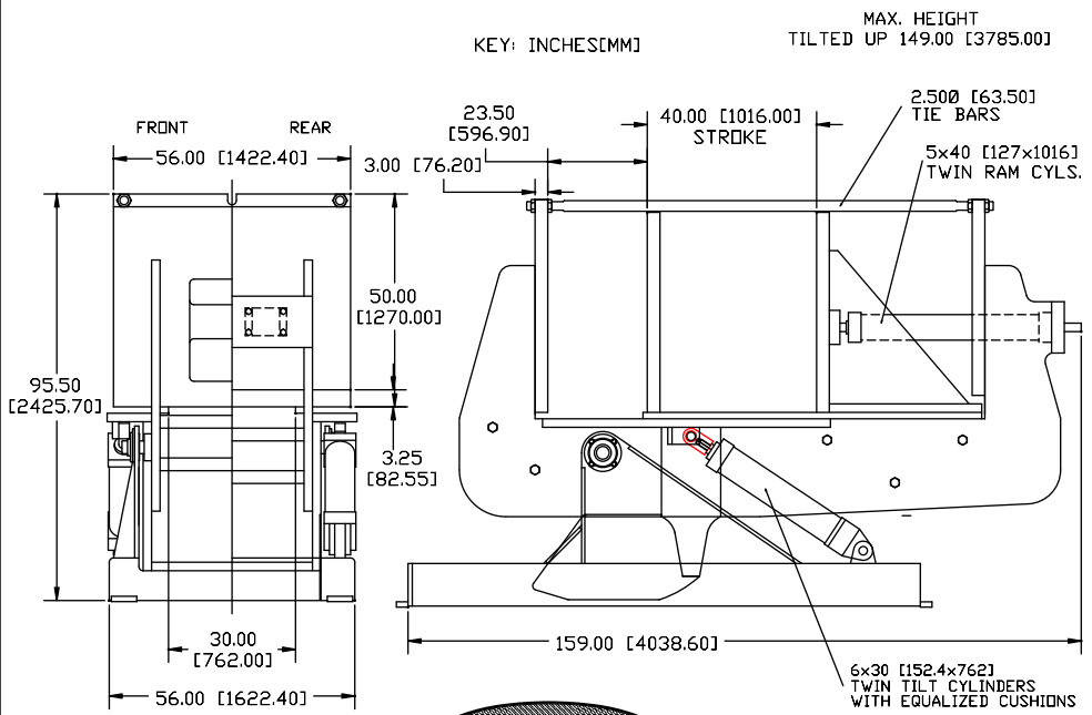
PLATEN, 3.00" MOVABLE
