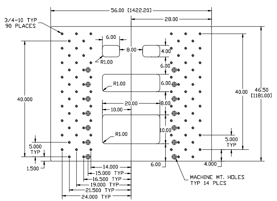
PLATEN, 3.00" MOVABLE
